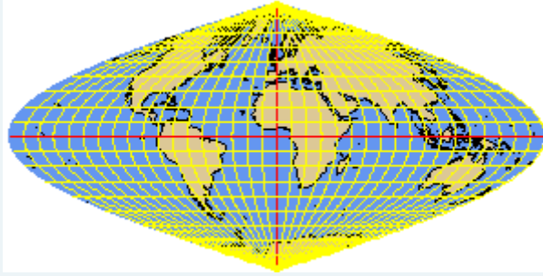
MERCANS sinusoidal (equal-area) projection or Mercator-Sanson-Flamsteed
